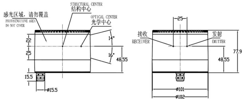
Figure 1.8 C16 Mechanical Drawing (unit: mm) (cable interface at bottom)
