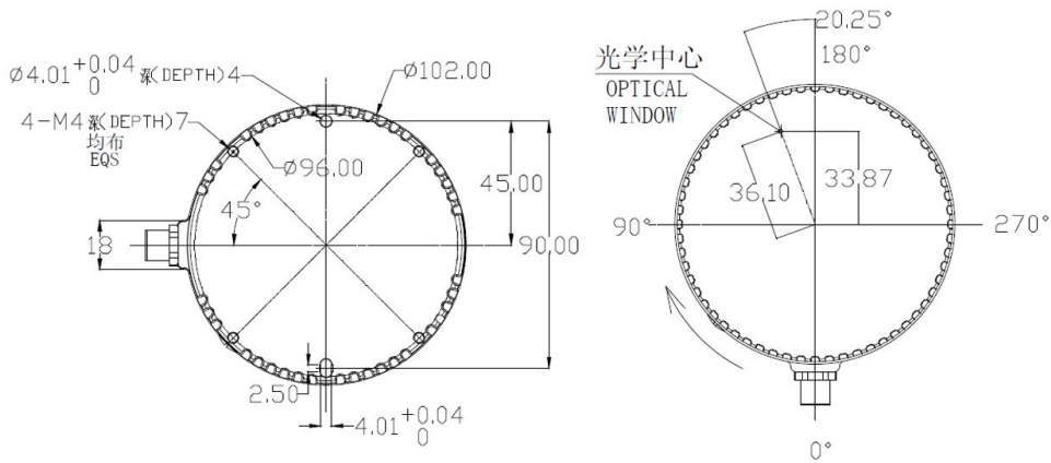
Figure 1.5 C16 Lidar Base (unit: mm) (cable interface at side)
