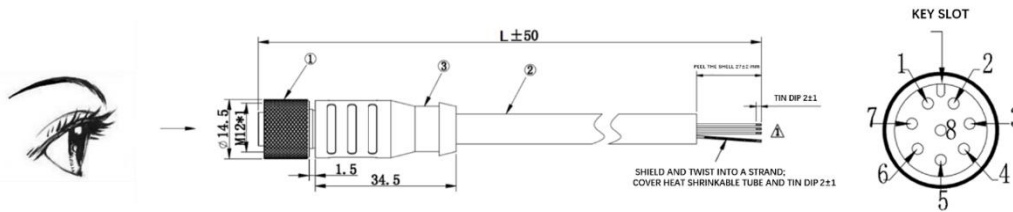
Figure 2.5 C16 Lidar Extension Cable (unit: mm)
