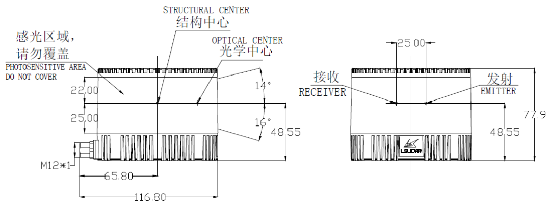
Figure 1.7 C16 Mechanical Drawing (unit: mm) (cable interface at side)
