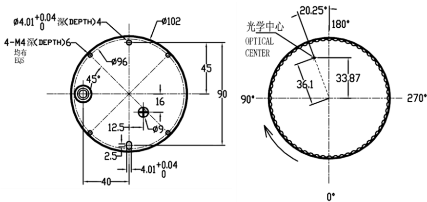
Figure 1.6 C16 Lidar Base (unit: mm) (cable interface at bottom)
