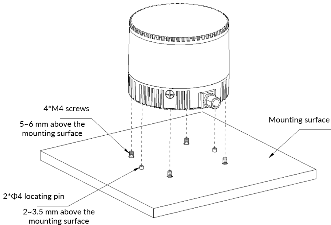
Figure 1.9 Mounting Reference Drawing
