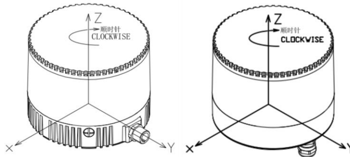
Figure 1.3 Coordinates & Scanning Direction (left: side; right: bottom)
