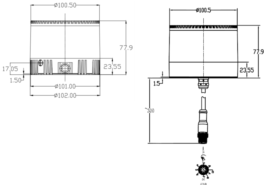
Figure 1.4 C16 Dimensions (unit: mm) (left: side; right: bottom)
